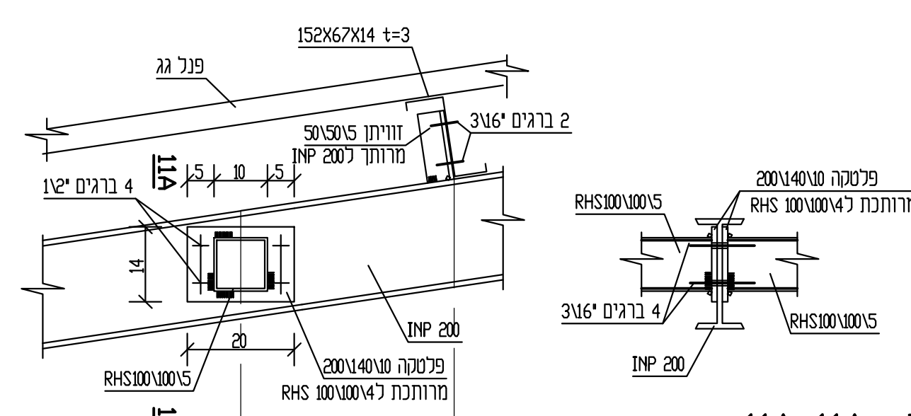
1:10 11A-11A חתך
